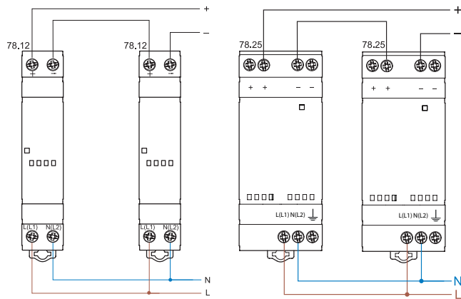
Series connection
