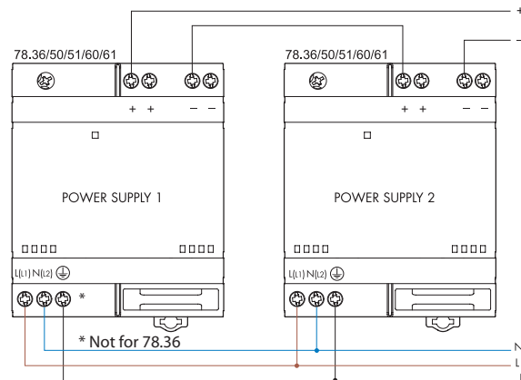
Series connection
