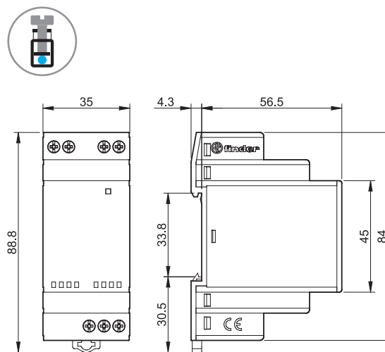
Types 78.50 / 78.60 Screw terminal
