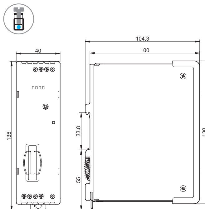
Type 78.1B Screw terminal
