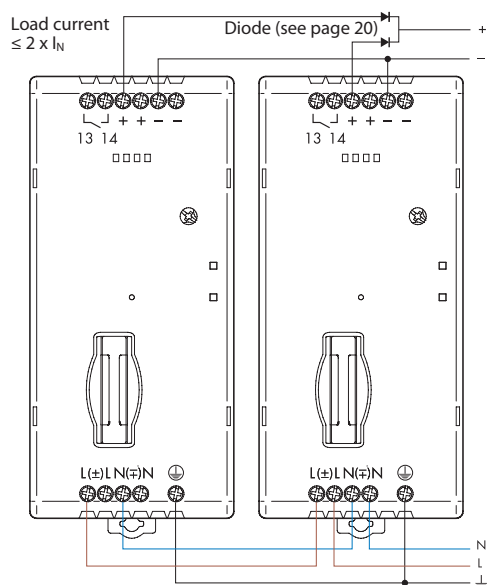
Parallel connection
