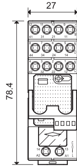
Type 58.34 Screw terminals
