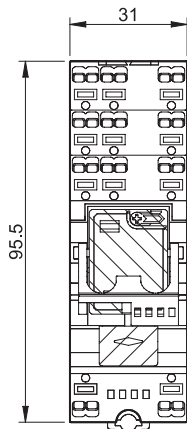
Type 58.P3 Push-in terminal
