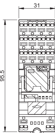
Type 58.P4 Push-in terminal
