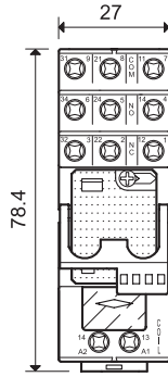
Type 58.33 Screw terminals
