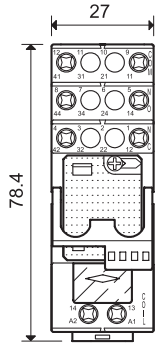
Type 58.32 Screw terminals
